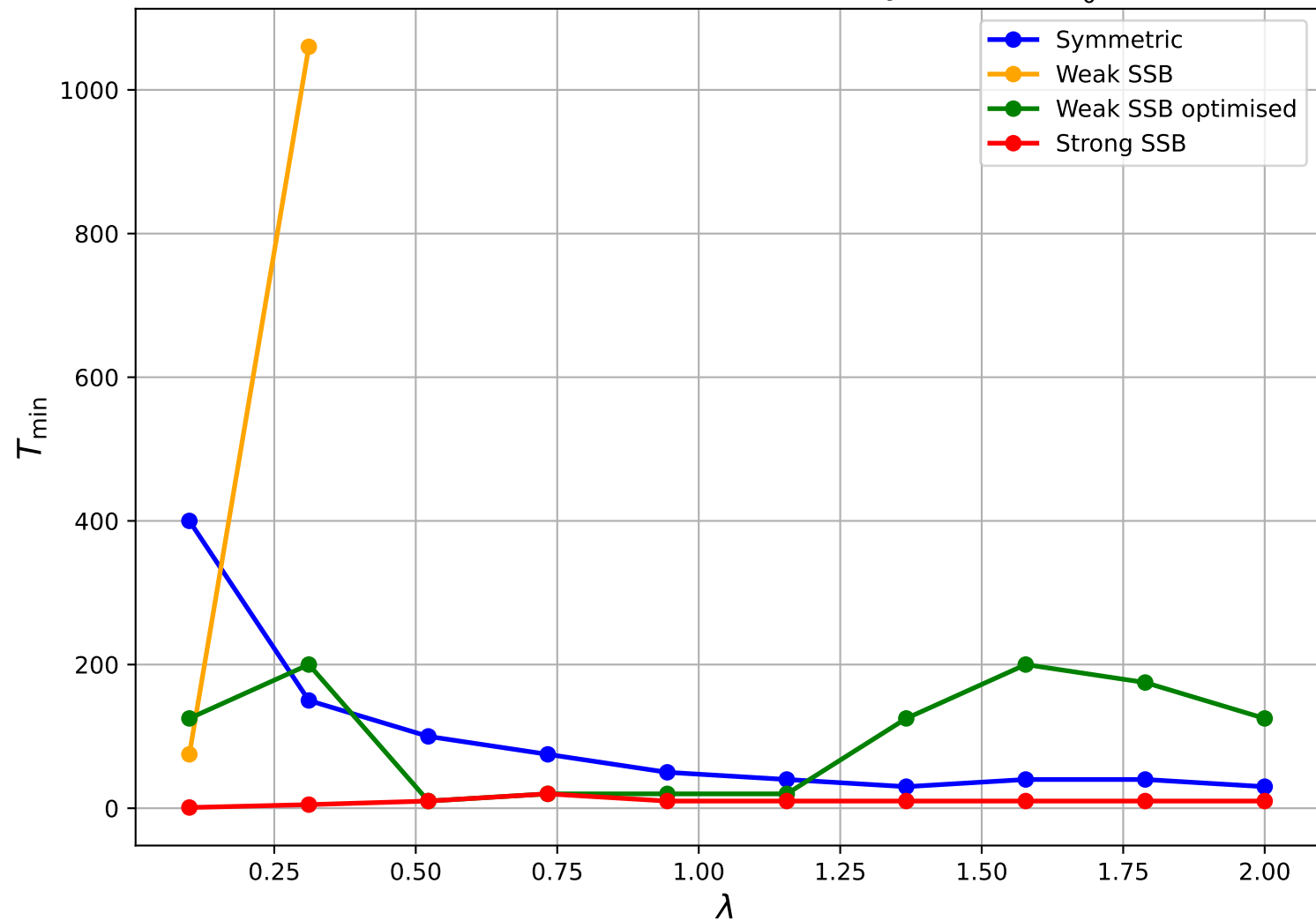
Minimum Adiabatic Time T_{\min} for Fidelity \geq 0.97 , m_0^2 = -2.0
